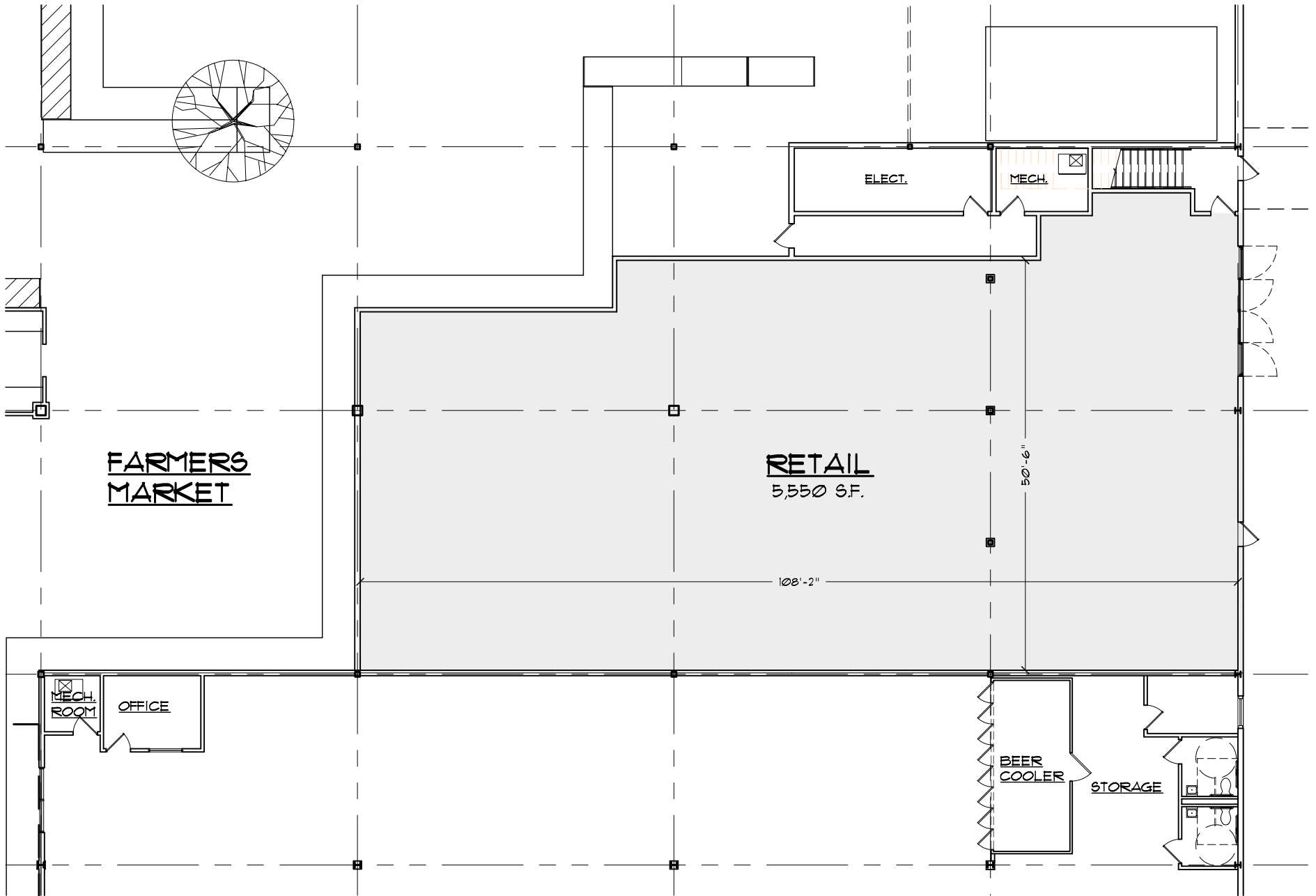
1 PARTIAL PLAN
